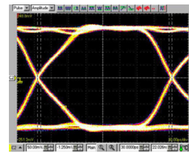
3EH-15G with Fixture: pin#4-pin#8 Rise Time: \approx 30\text{ps} , Bit Rate: 4.25\text{Gb/s} PRBS (Pseudo Random Bit Sequence): 2^{10}-1
