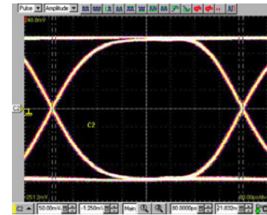
3EH-15G with Fixture: pin#4-pin#10 Rise Time: \approx 250\text{ps} , Bit Rate: 1.6\text{Gb/s} PRBS (Pseudo Random Bit Sequence): 2^{10}-1
