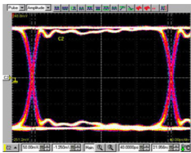
Through Fixture Rise Time: \approx 30\text{ps} , Bit Rate: 3.2\text{Gb/s} PRBS (Pseudo Random Bit Sequence): 2^{10}-1
