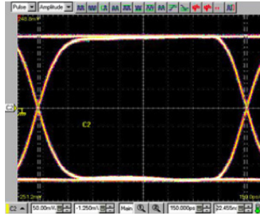
3EH-15G with Fixture: pin#4-pin#8 Rise Time: \approx 250\text{ps} , Bit Rate: 800\text{Mb/s} PRBS (Pseudo Random Bit Sequence): 2^{10}-1
