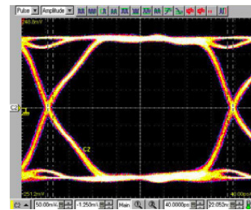
3EH-15G with Fixture: pin#4-pin#8 Rise Time: \approx 30\text{ps} , Bit Rate: 3.2\text{Gb/s} PRBS (Pseudo Random Bit Sequence): 2^{10}-1
