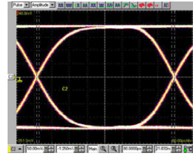
3EH-15G with Fixture: pin#4-pin#8 Rise Time: \approx 250\text{ps} , Bit Rate: 1.6\text{Gb/s} PRBS (Pseudo Random Bit Sequence): 2^{10}-1
