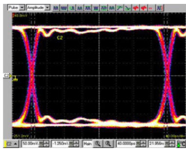
Through Fixture Rise Time: \approx 30\text{ps} , Bit Rate: 3.2\text{Gb/s} PRBS (Pseudo Random Bit Sequence): 2^{10}-1
