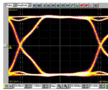
3EH-15G with Fixture: pin#4-pin#10 Rise Time: \approx 30\text{ps} , Bit Rate: 3.2\text{Gb/s} PRBS (Pseudo Random Bit Sequence): 2^{10}-1
