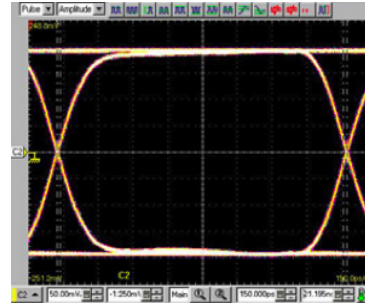
3EH-15G with Fixture: pin#4-pin#10 Rise Time: \approx 250\text{ps} , Bit Rate: 800\text{Mb/s} PRBS (Pseudo Random Bit Sequence): 2^{10}-1
