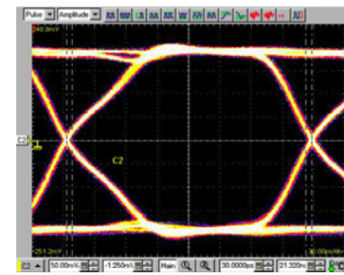
3EH-15G with Fixture: pin#4-pin#10 Rise Time: \approx 30\text{ps} , Bit Rate: 4.25\text{Gb/s} PRBS (Pseudo Random Bit Sequence): 2^{10}-1
