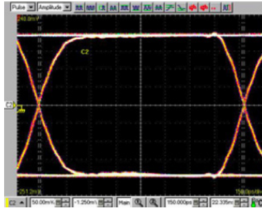
Through Fixture Rise Time: \approx 250\text{ps} , Bit Rate: 800\text{Mb/s} PRBS (Pseudo Random Bit Sequence): 2^{10}-1
